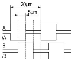
Fig. 2: Output of the quadrature signals
