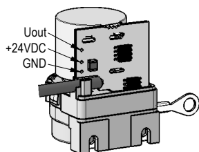
Fig. 7: Potentiometer connection MWU
