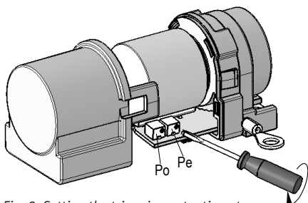
Fig. 8: Setting the trimming potentiometers
